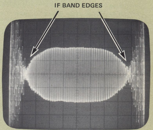
Figure 5. Dual Sweep Response (Detector Alignment)
