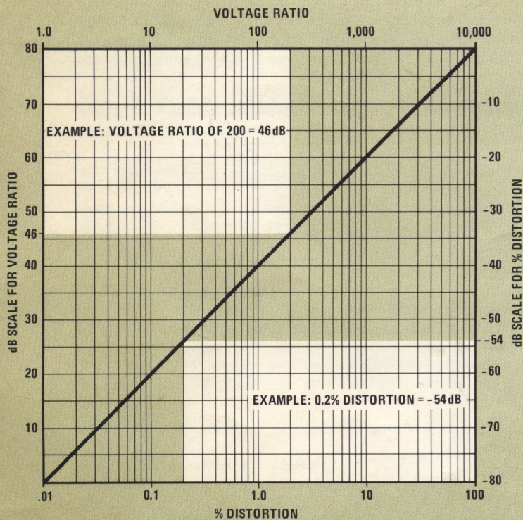
dB CONVERSION
