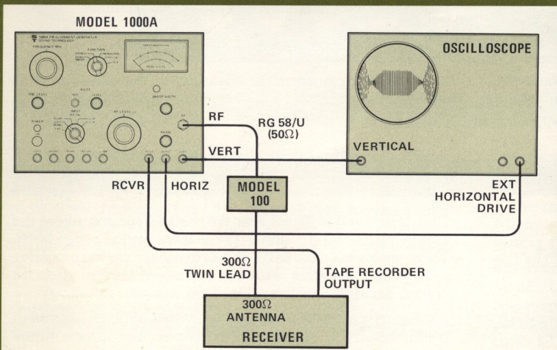
Figure 2. Discriminator Alignment
