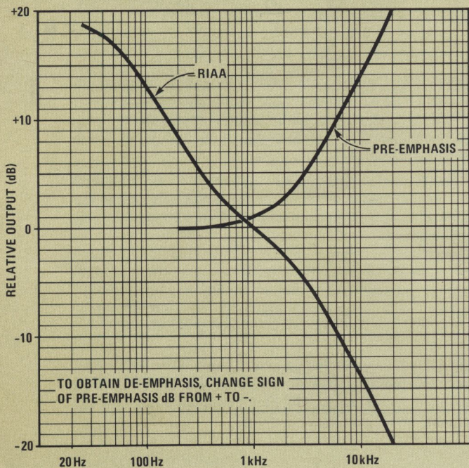
EQUALIZATION CURVES
