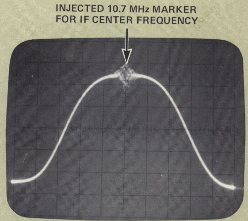
Figure 4. RF and IF Response
