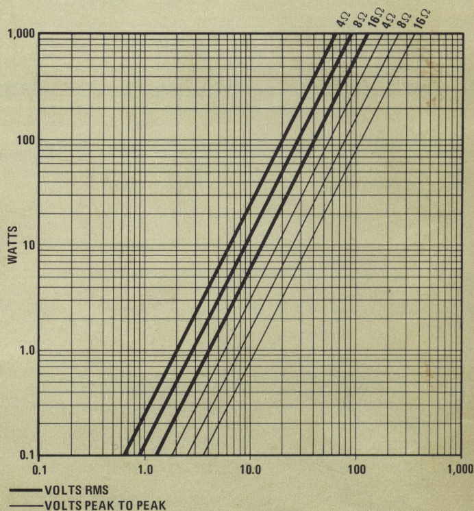
VOLTAGE-TO-POWER CONVERSION
