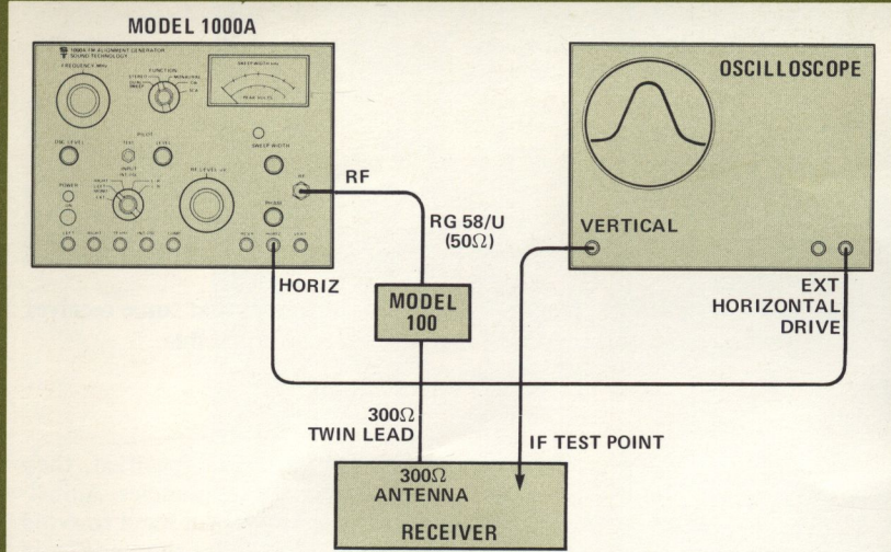
Figure 1. RF and IF Sweep Alignment
